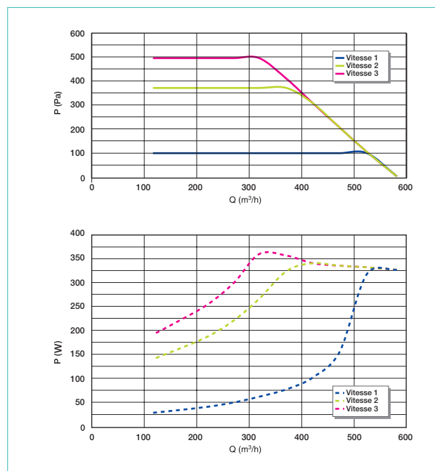
Constate druk
